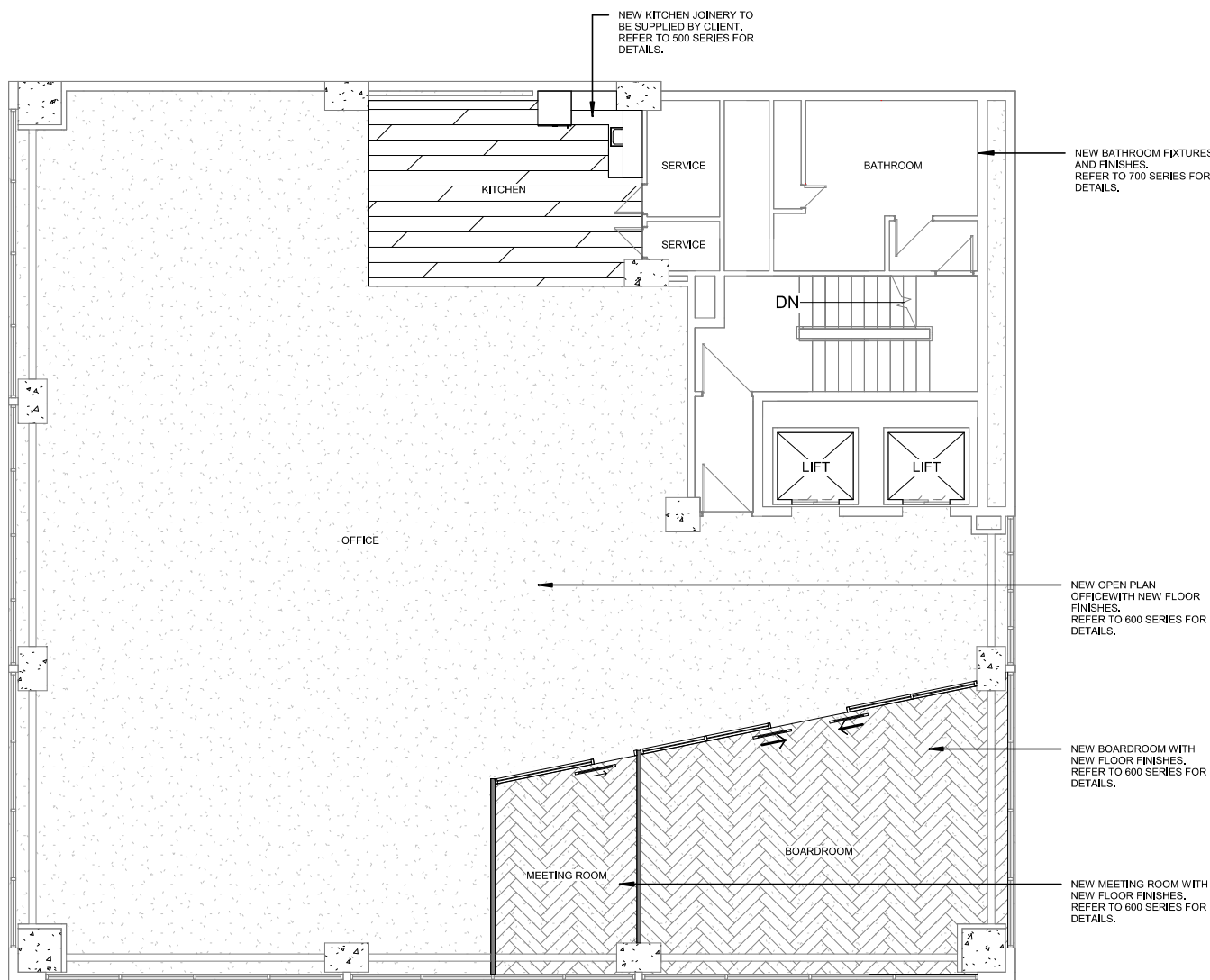
1 250-01 250 01 PROPOSED OFFICE GENERAL ARRANGEMENT PLAN (L4,L7,L10) 1 : 100
