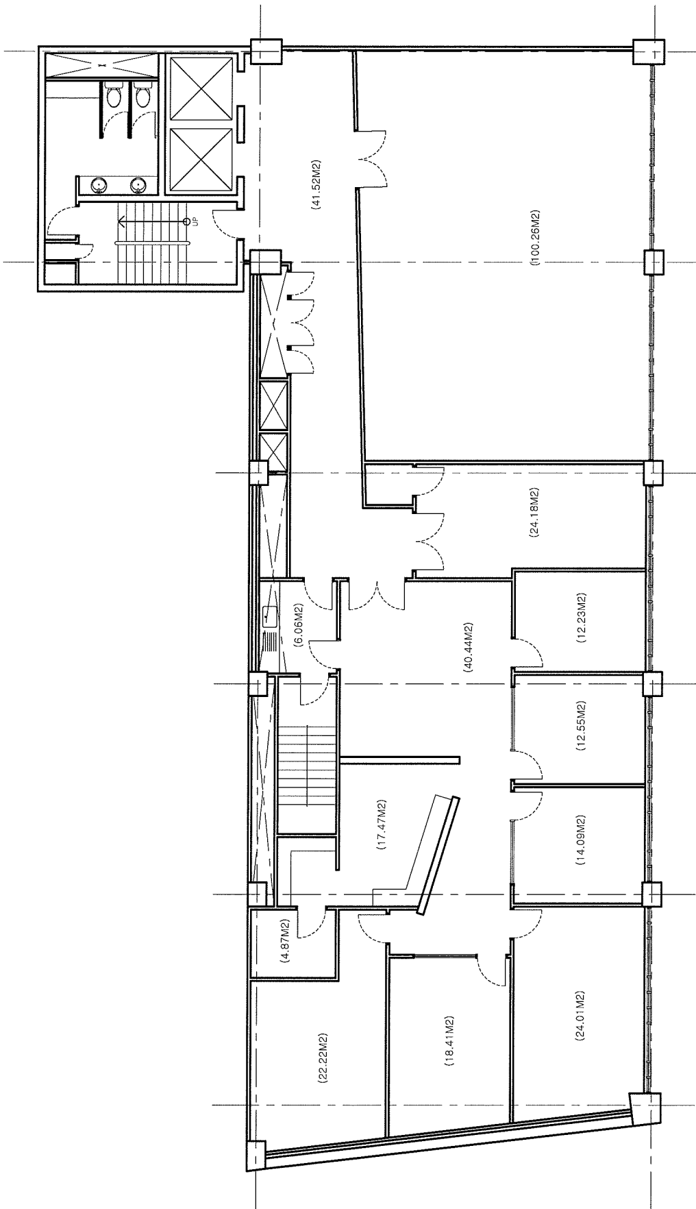
1ST FLOOR PLAN SCALE 1/100
